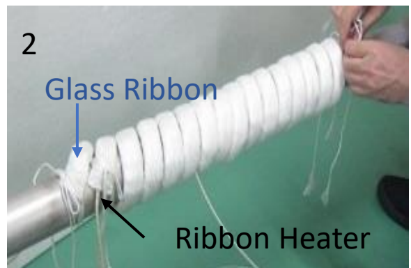
2 After installing the Ribbon heater, it is recommended to also install our Glass Ribbon too
