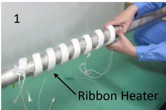
1 Installing the ribbon heater, without Glass ribbon and outer cloth
